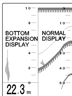
NORMAL DISPLAY & BOTTOM EXPANSION DISPLAY
