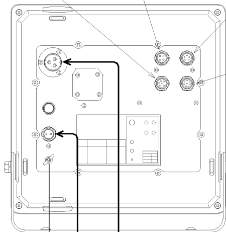
EXTERNAL SOUNDER -INTERFACE (8 pins)
