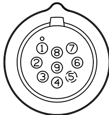
CONTACT END VIEW
