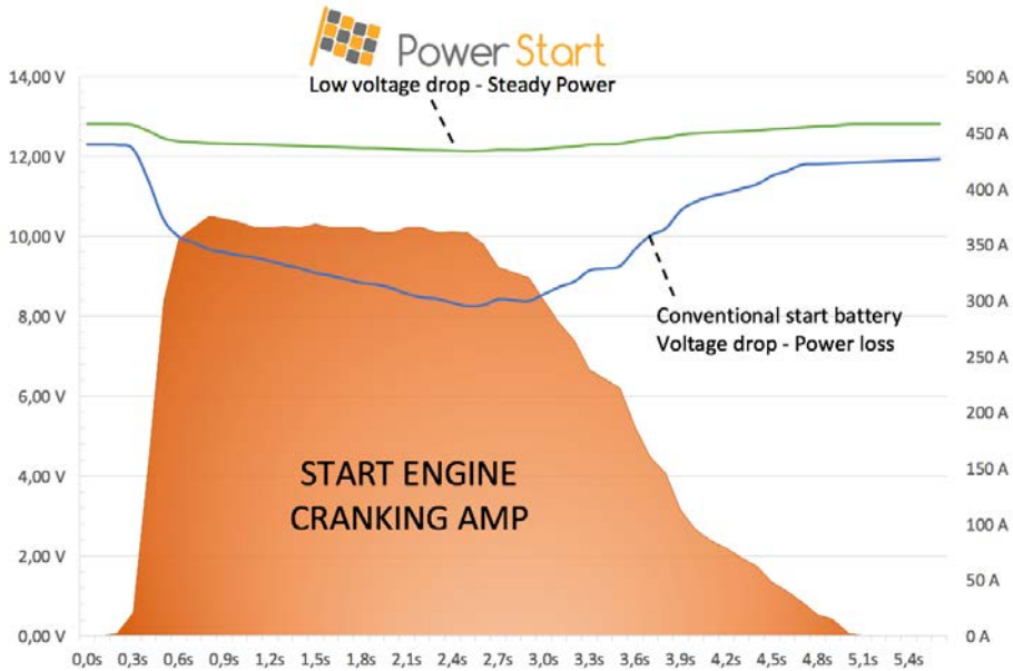
PowerStart Typical Start Cycle
